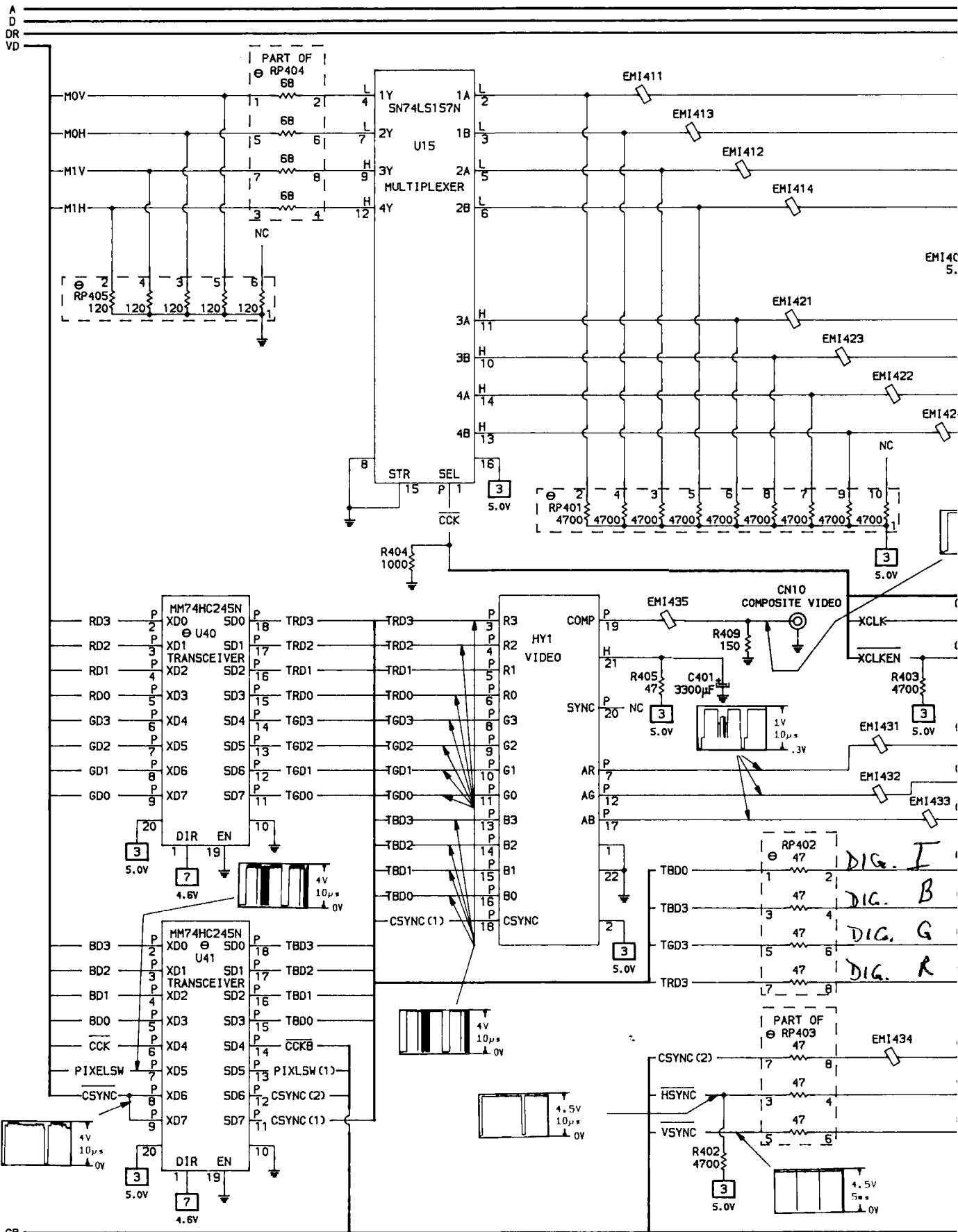
A PHOTOFACT STANDARD NOTATION SCHEMATIC WITH CIRCUITACE
